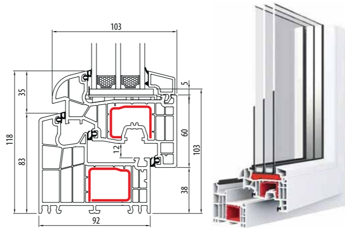
BluEvolution 92 Round-line
