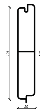
Bretterpaneel
