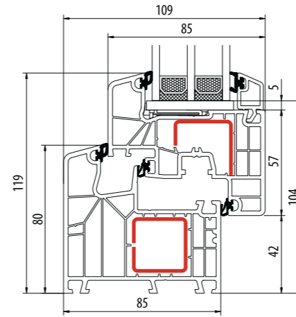
Ideal 8000 Classic-line
